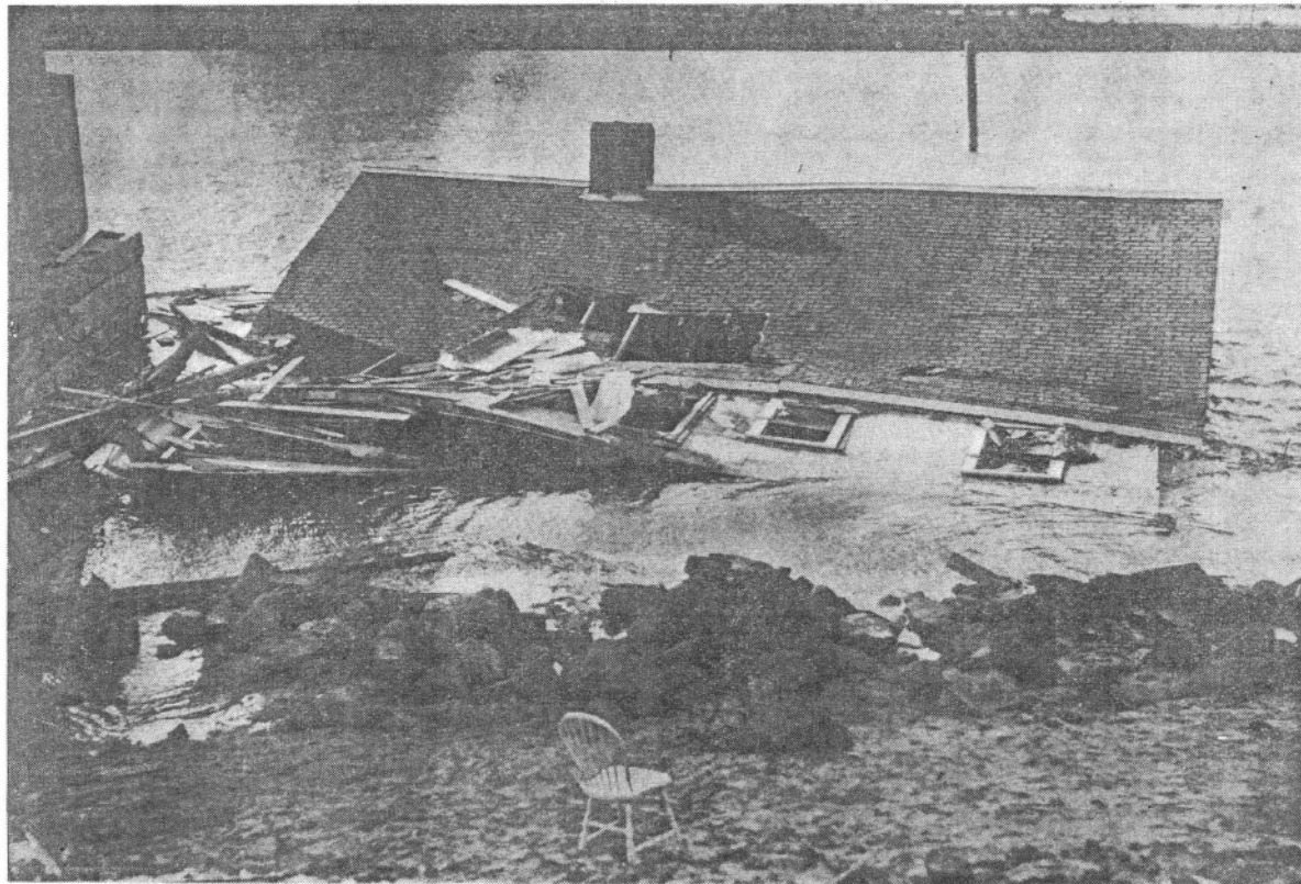
This house crumbled and slithered into the Cape Cod Canal during the hurricane and tidal wave, causing the death of five persons. The bodies of the victims were removed from the hole that can be seen in the roof. The wreckage crashed against the abutment of the Bourne Bridge shown at left.
